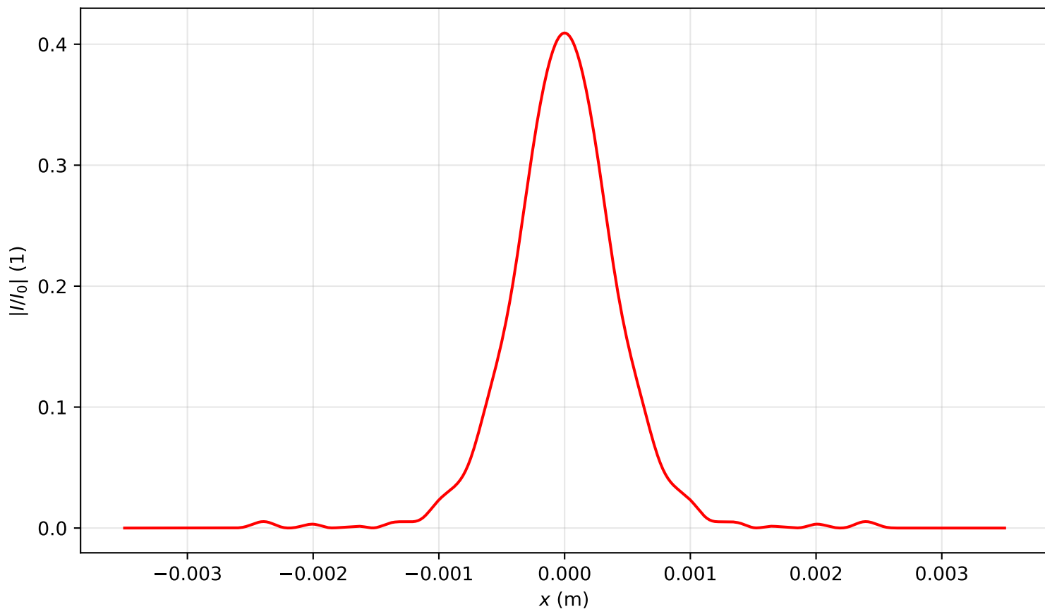
Intensity profile I(x, y = 0, z = 2.548)/I_0 , P_{in}=1.0P_{cr} , artificial time
